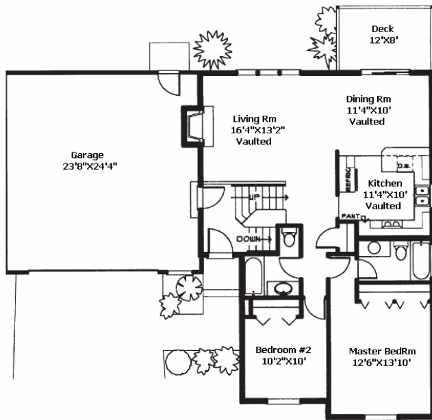
Main Floor
